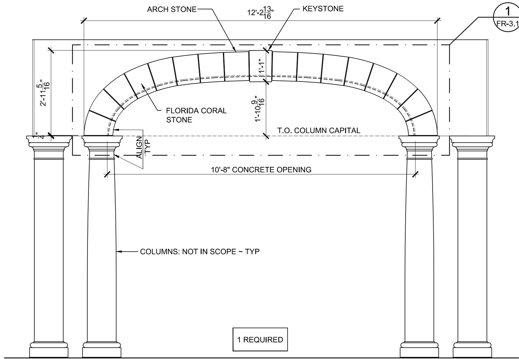
1 BREEZEWAY AT LOGGIA 113 FR-3.0 SCALE: 1/2"=1'-0"
